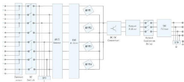
Circuit Diagram
